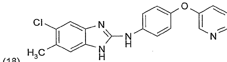
(18) (5-Chloro-6-methyl-1H-benzimidazol-2-yl)-[4-(pyridin-3-yloxy)-phenyl]-amin
